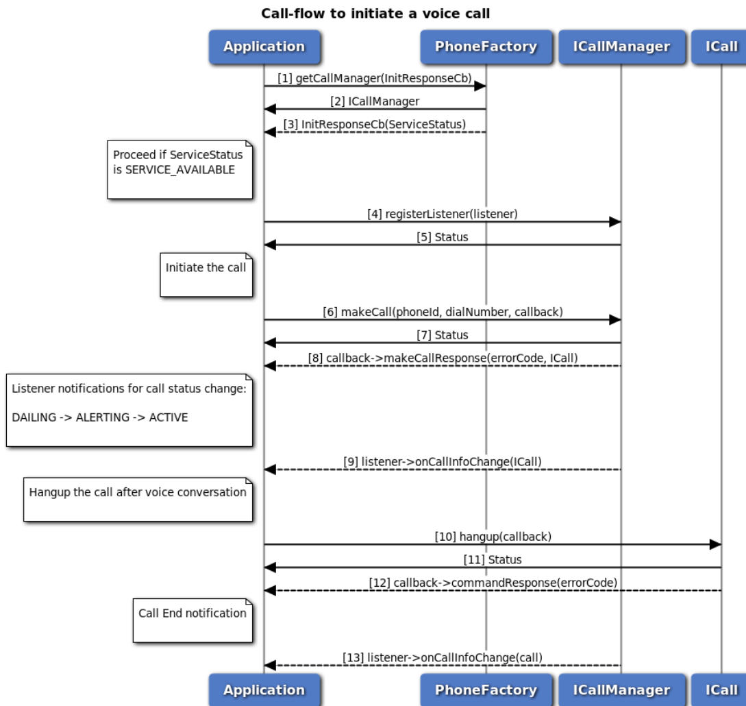
Figure 3-2 Dial call flow
