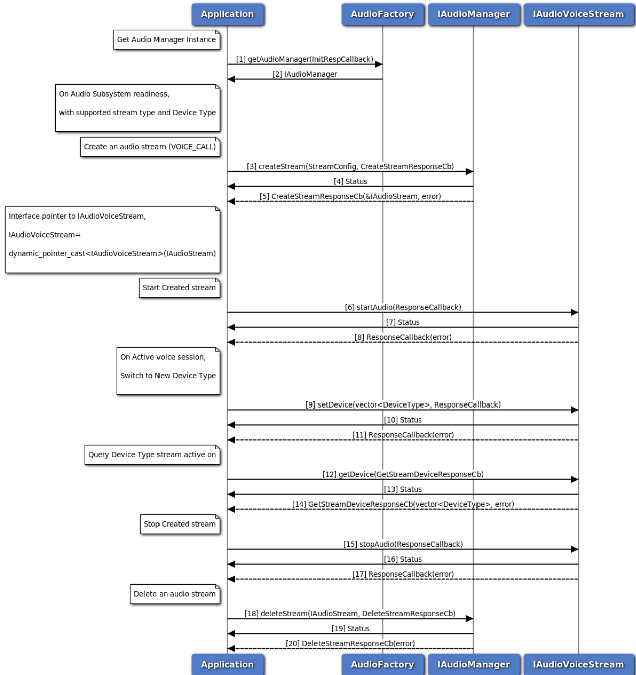
Figure 3-100 Audio Voice Call Device Switch call flow
