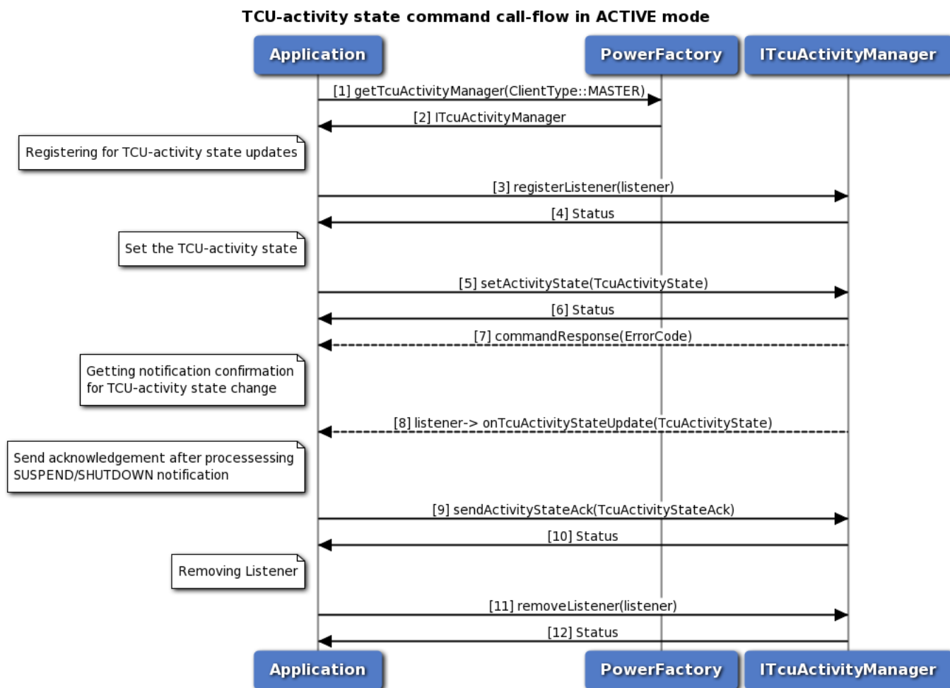
Figure 3-116 Call flow to set the TCU-activity state in ACTIVE mode
