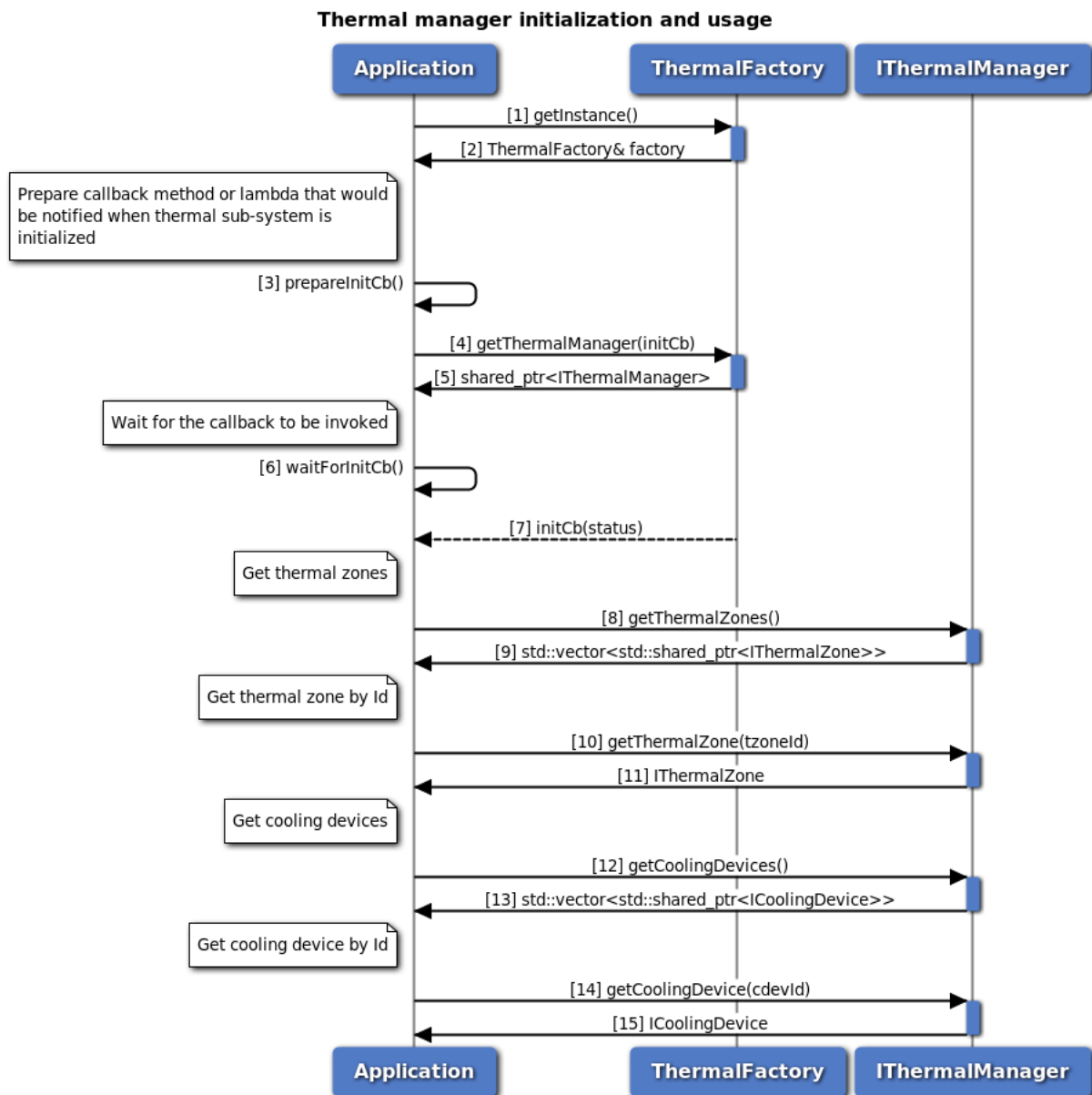
Figure 3-111 Thermal manager call flow
