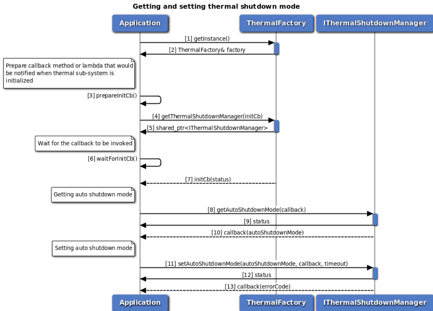
Figure 3-113 Call flow to set/get the Thermal auto-shutdown mode
