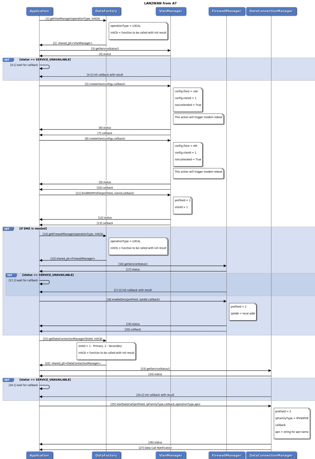
Figure 3-63 LAN-WAN VLAN Configuration Usecase from A7 call flow
