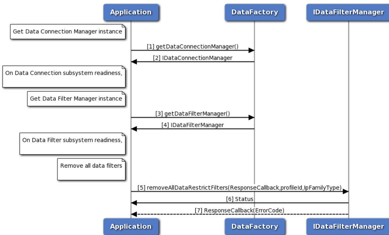
Figure 3-53 Remove data restrict filter call flow
