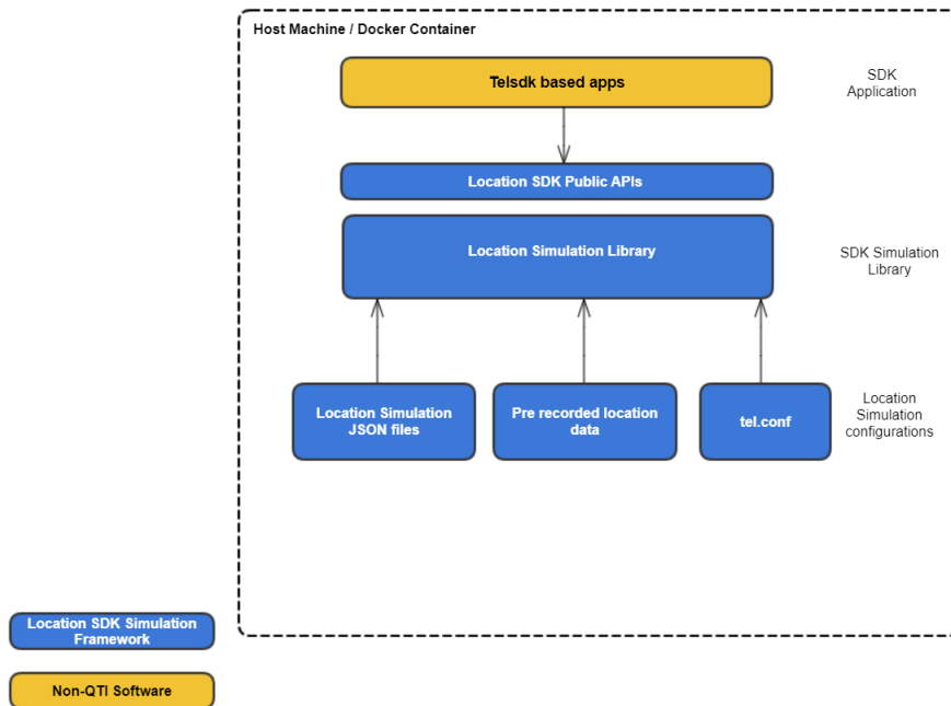
Figure 3-4 Location Simulation Framework
