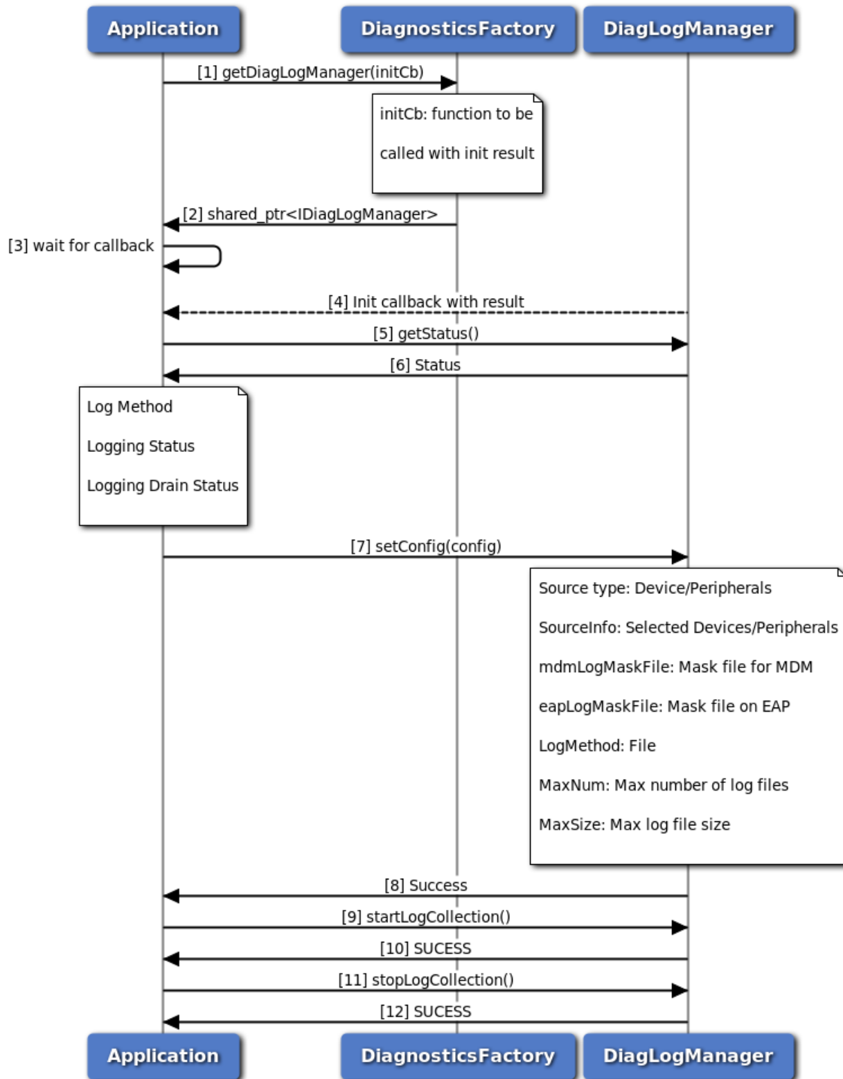
Figure 3-149 Log Collection Using File Method Call Flow
