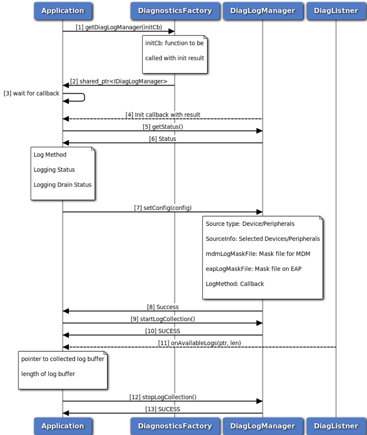
Figure 3-150 Log Collection Using Callback Method Call Flow
