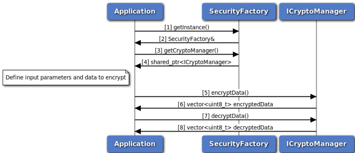
Figure 3-137 Call flow to encrypt and decrypt data
