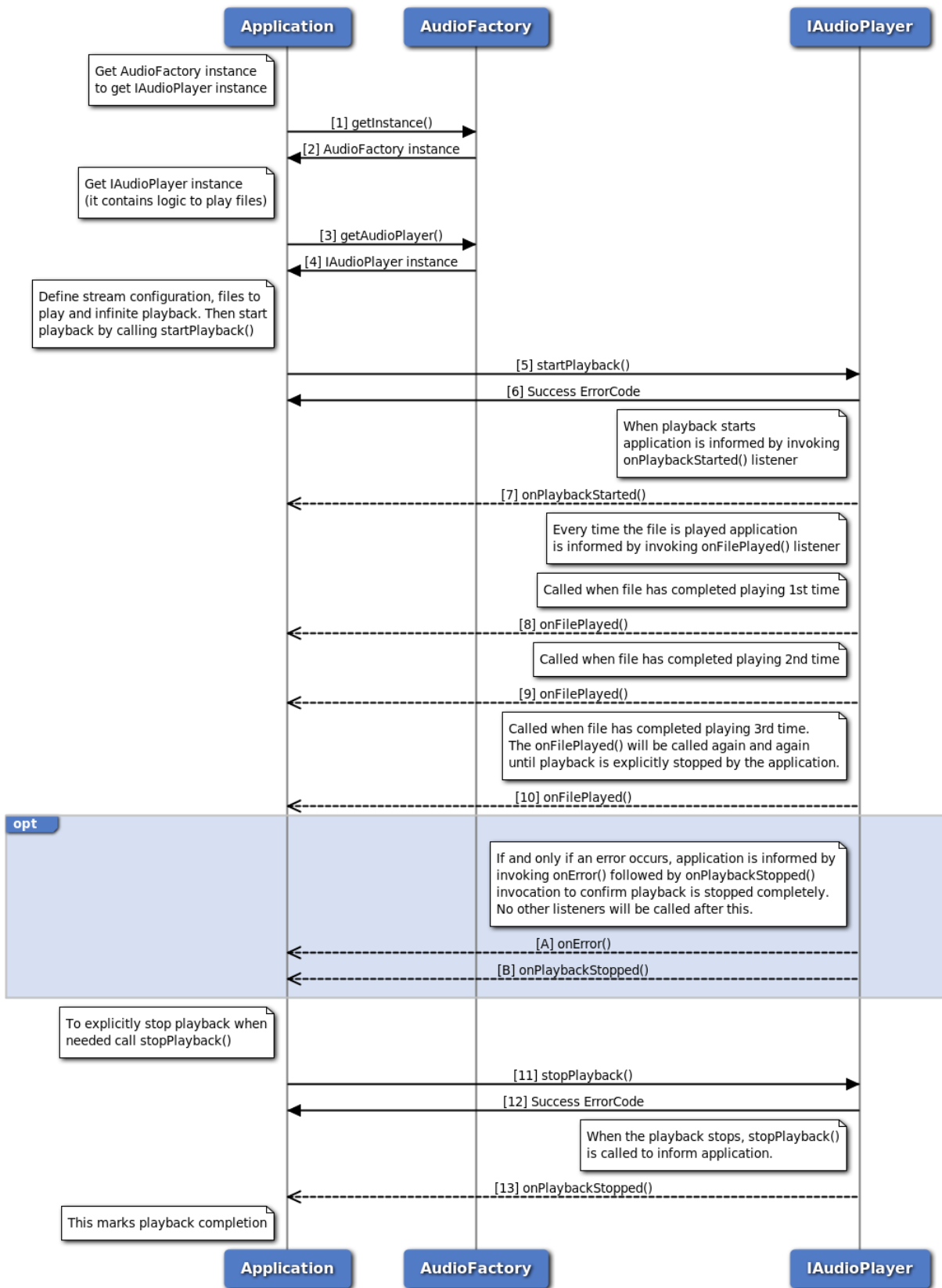
Figure 3-114 Playing a file indefinitely call flow
