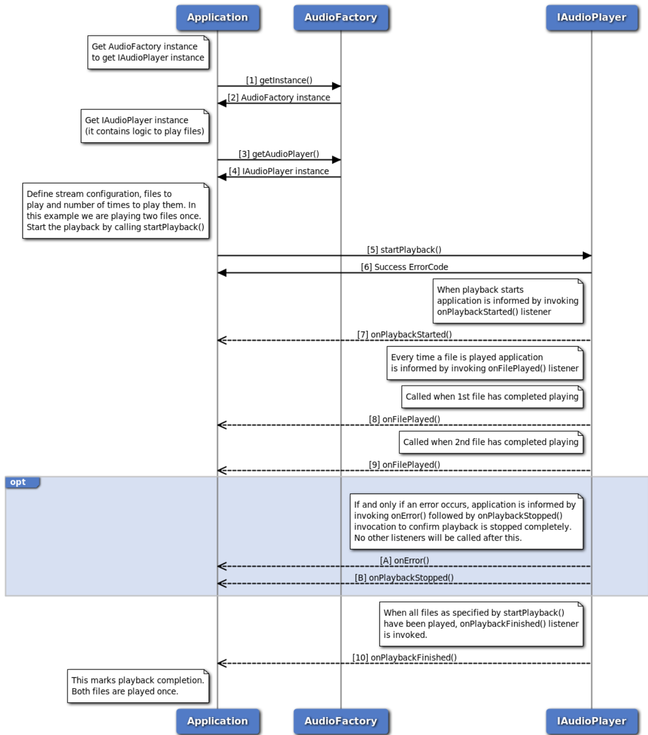
Figure 3-113 Playing a file specific number of times call flow
