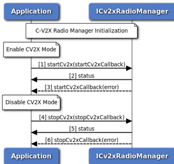
Figure 3-76 Start/Stop C-V2X Mode Call Flow - C++ Version
