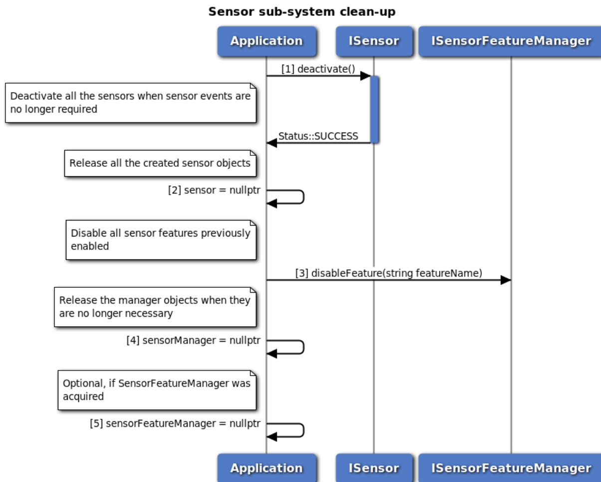
Figure 3-128 Sensor sub-system cleanup call flow
