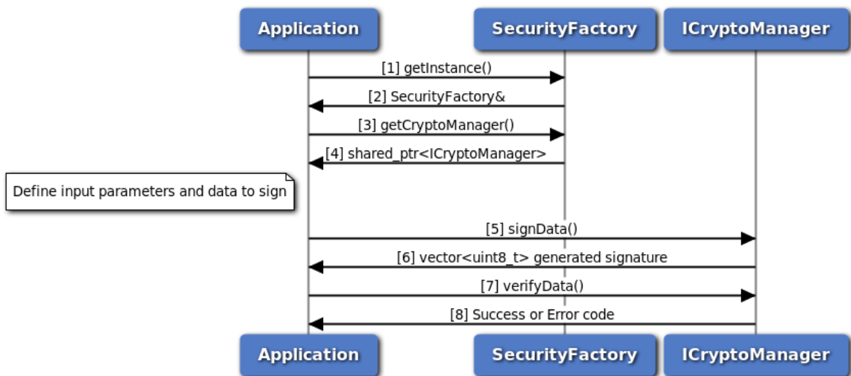
Figure 3-136 Call flow to sign and verify data
