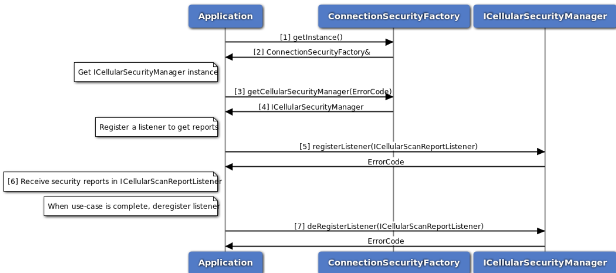
Figure 3-144 Call flow to register listener and receive reports
