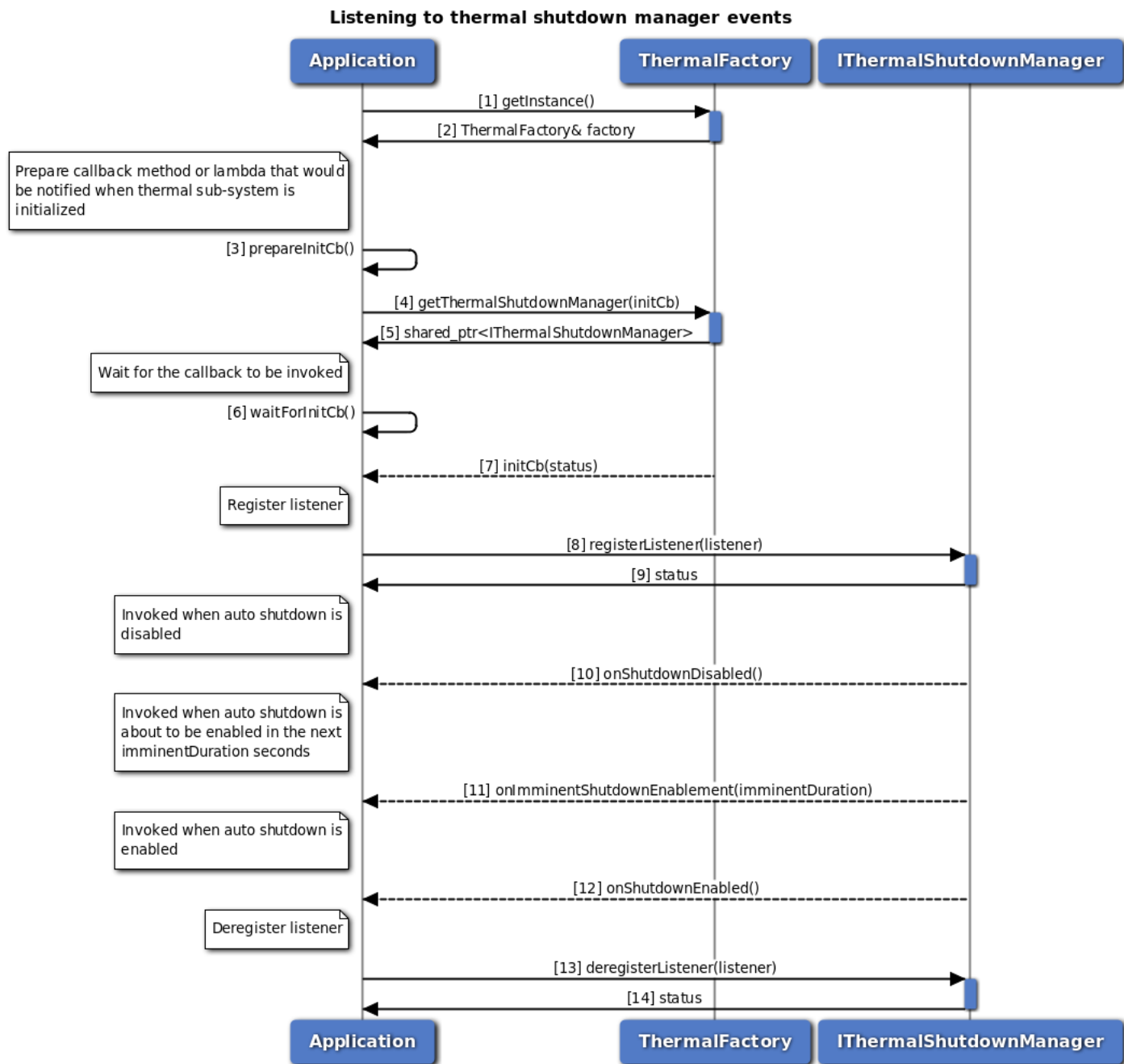
Figure 3-117 Call flow to register/remove listener for Thermal shutdown manager
