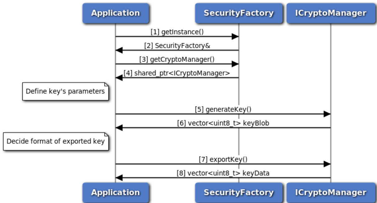
Figure 3-135 Call flow to generate and export key
