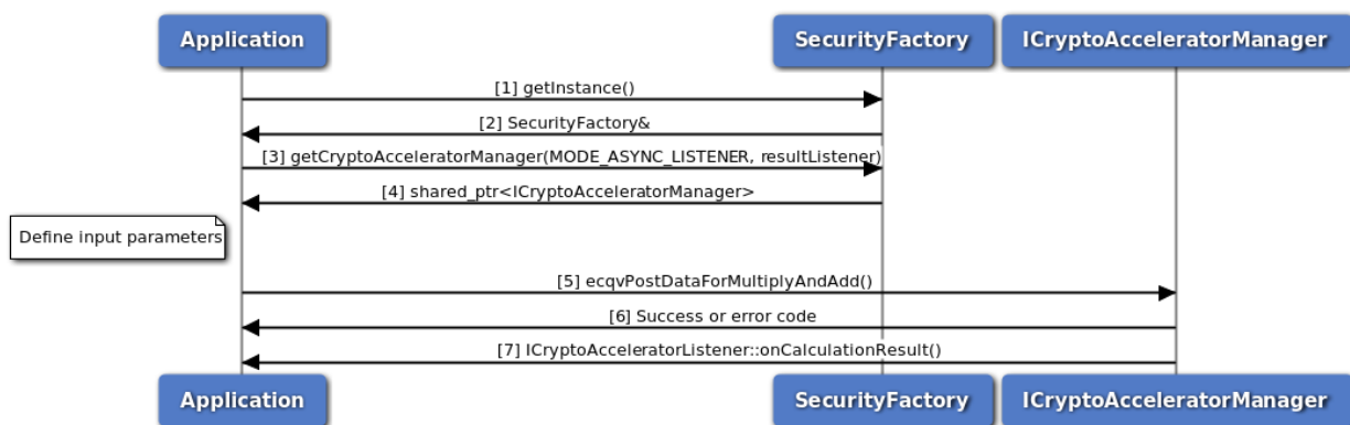
Figure 3-143 Call flow for ECQV calculation asynchronous listener mode
