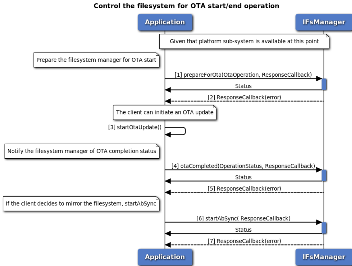
Figure 3-133 Control the filesystem for OTA operation call flow
