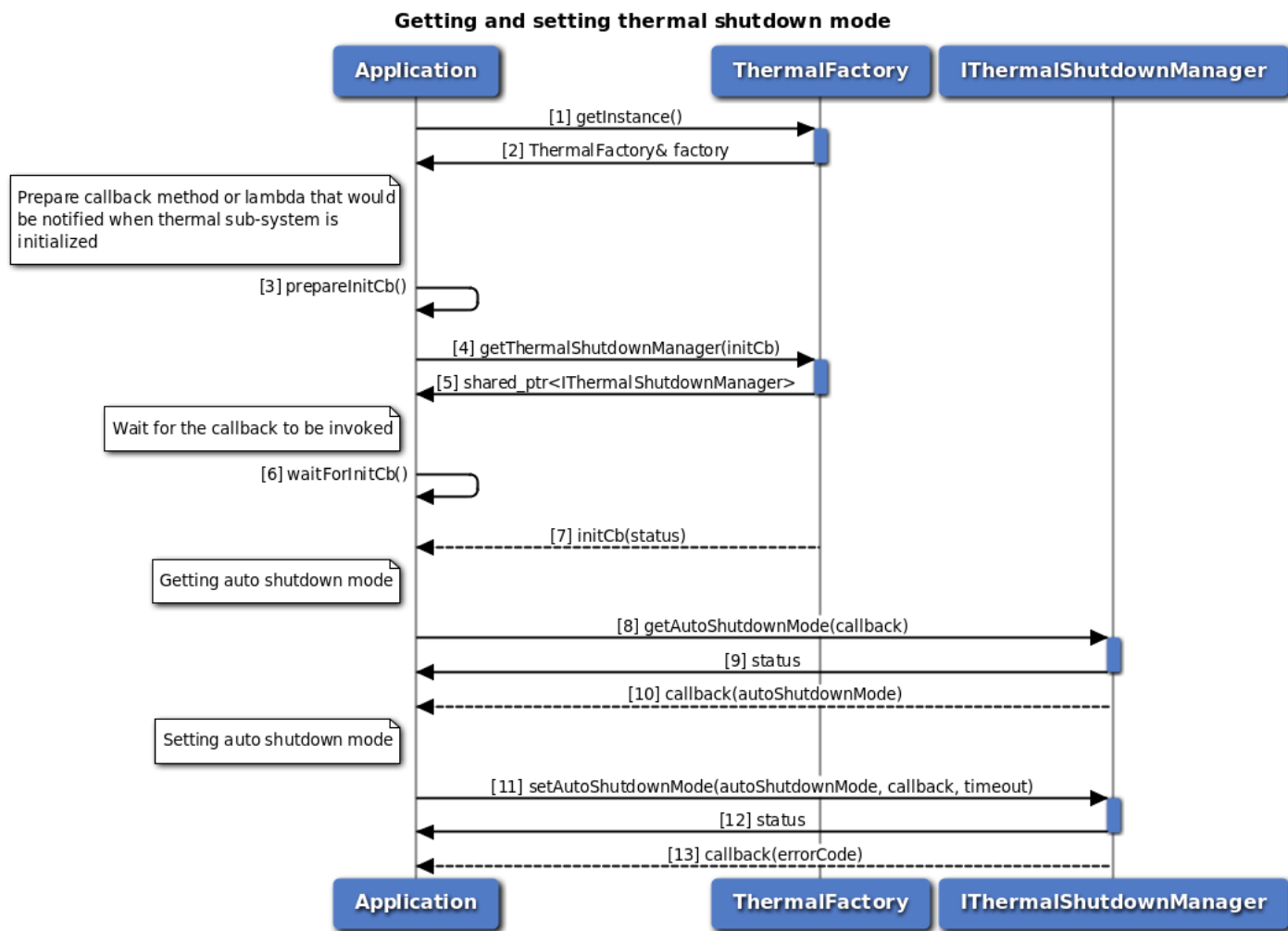
Figure 3-118 Call flow to set/get the Thermal auto-shutdown mode
