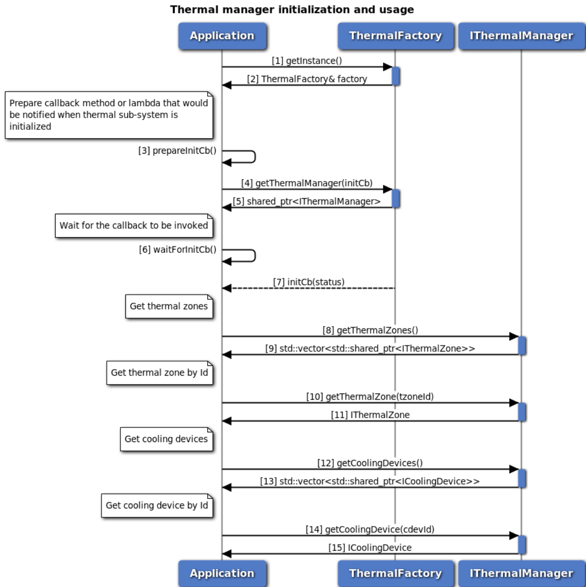
Figure 3-115 Thermal manager API call flow
