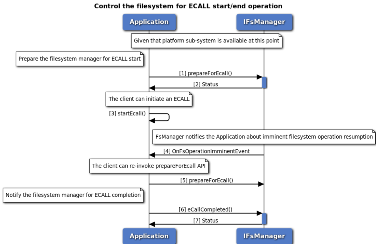
Figure 3-132 Control the filesystem for ECALL operation call flow
