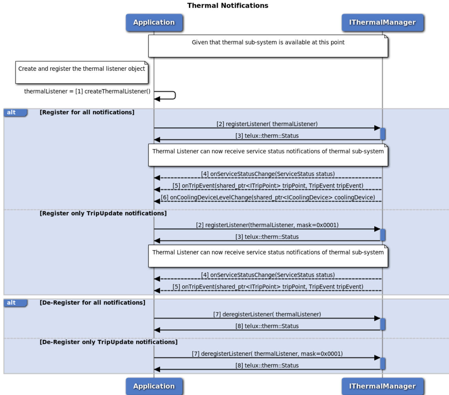
Figure 3-116 Call flow to register/remove listener for Thermal manager notifications
