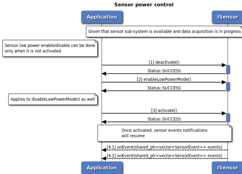
Figure 3-129 Sensor power control cleanup call flow
