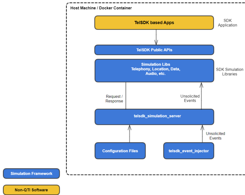
Figure 3-2 TeISDK Simulation Architecture
