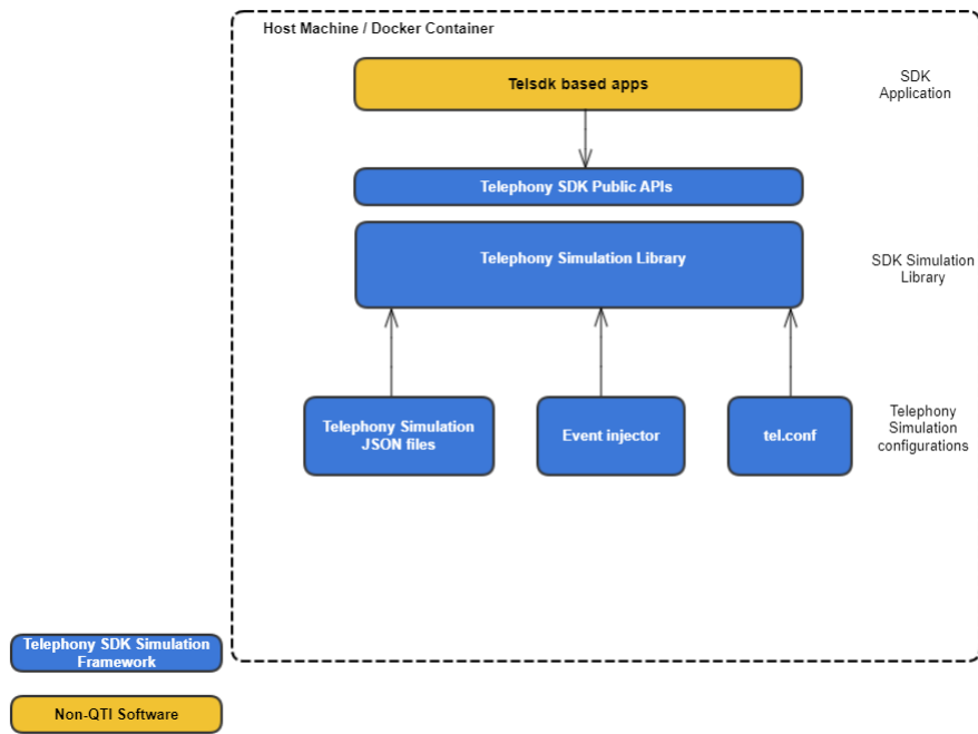
Figure 3-3 Telephony Simulation Framework
