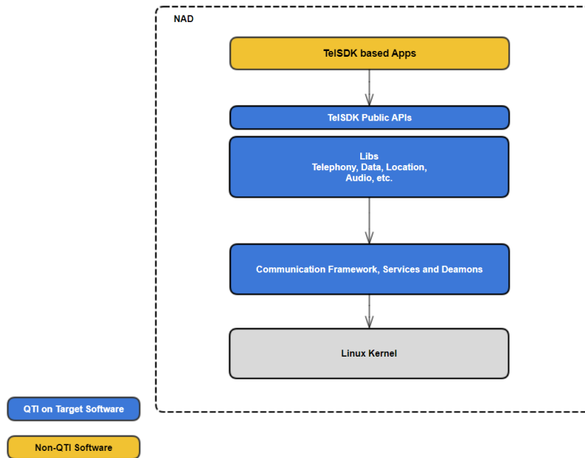
Figure 3-1 TelSDK On-Target Architecture
