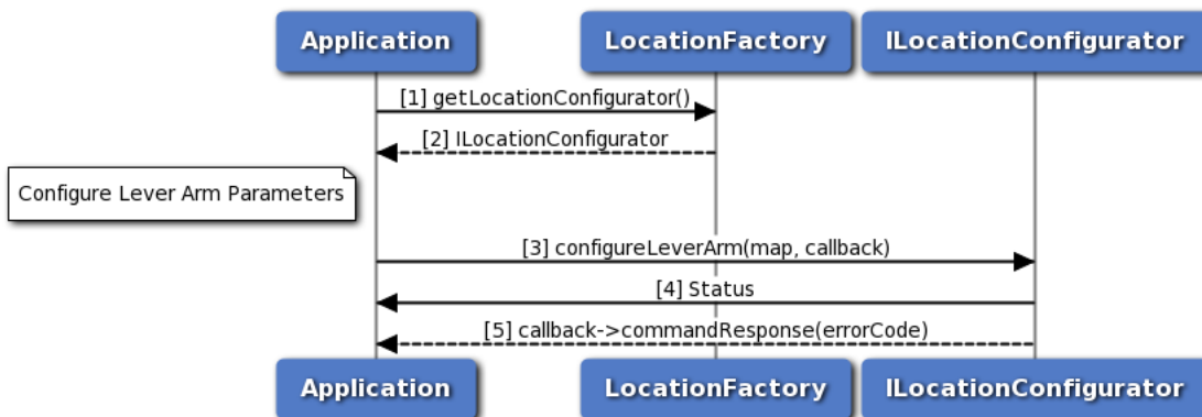
Figure 3-36 Call flow to configure lever arm parameters
