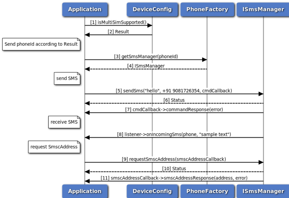
Figure 3-8 SMS call flow
