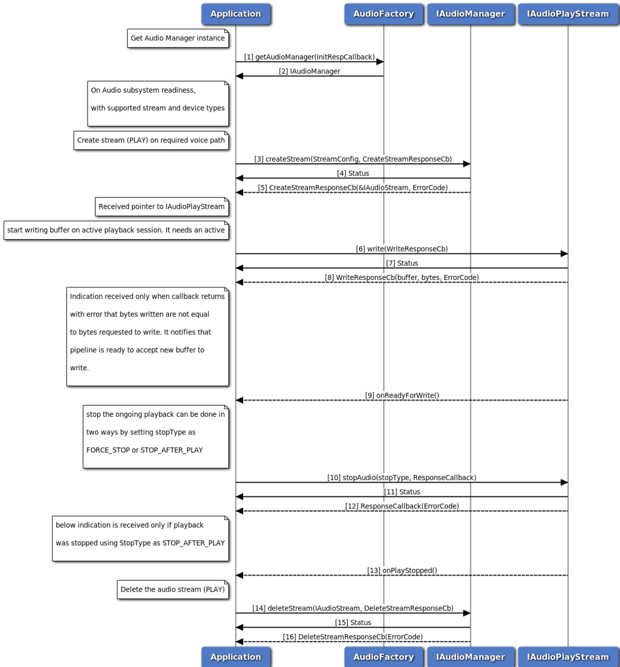
Figure 3-109 Compressed audio format playback on Voice Paths Callflow
