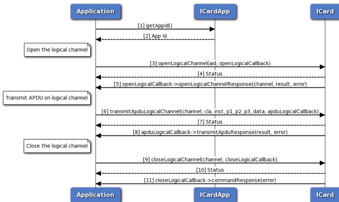
Figure 3-18 On logical channel
