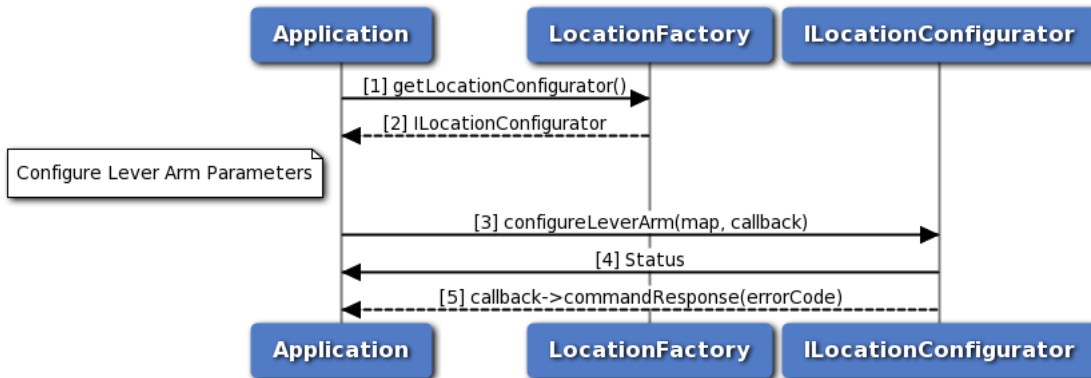
Figure 3-35 Call flow to configure lever arm parameters
