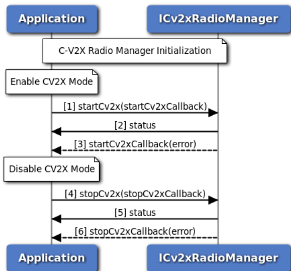
Figure 3-75 Start/Stop C-V2X Mode Call Flow - C++ Version
