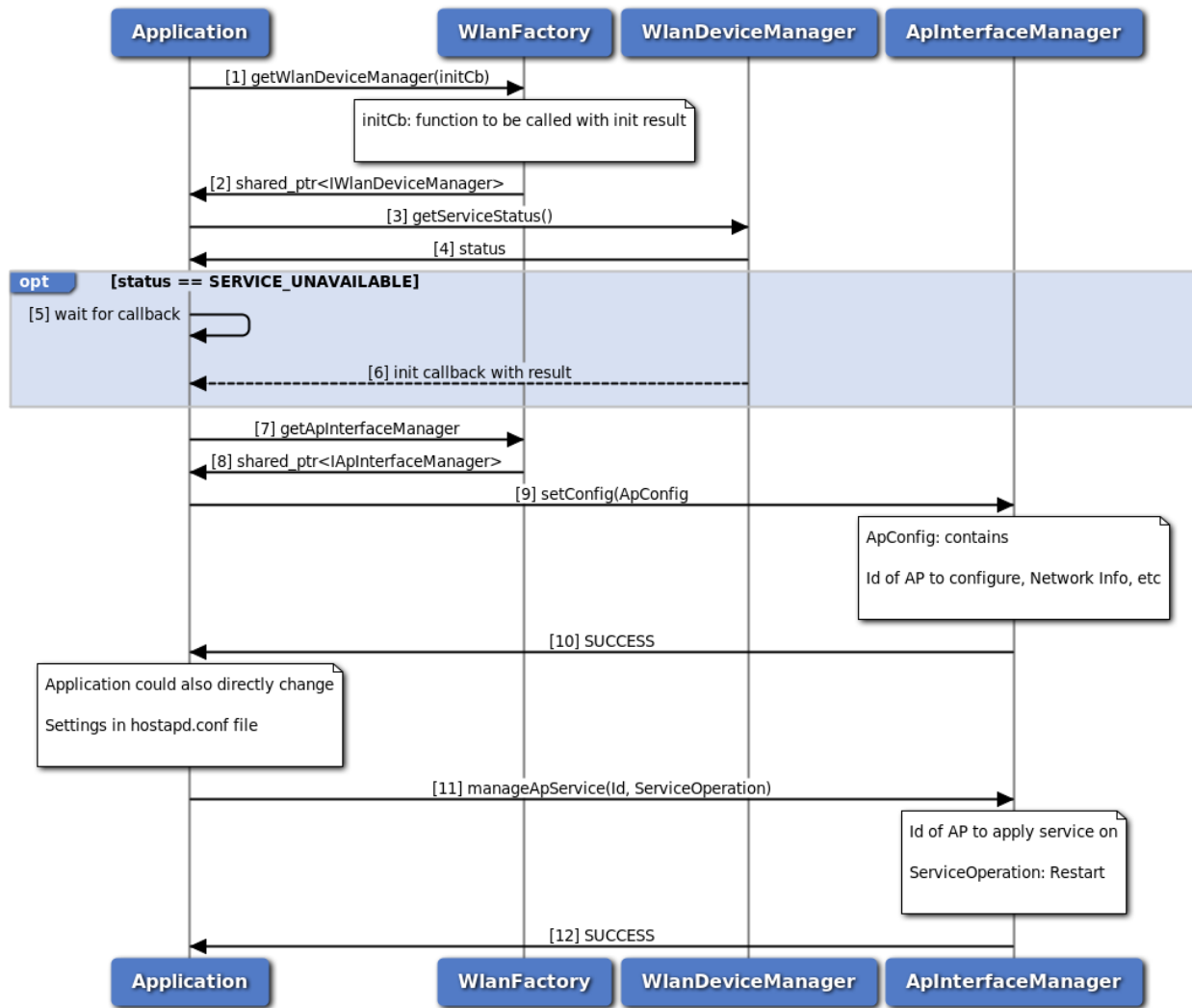
Figure 3-145 Modify WLAN Access Point Configuration Call Flow
