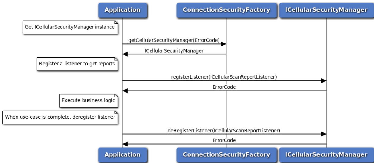
Figure 3-141 Call flow to register listener and receive reports
