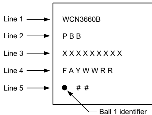
Figure 2-1 WCN3660B part marking (top view, not to scale)
